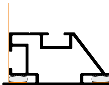
Assembly 2 textile sides with silicone
