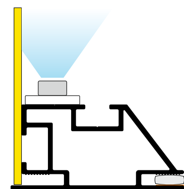
Assembly 1 textile side with perimeter LED
