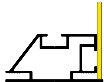
Assembly with 3mm rigid panel front
