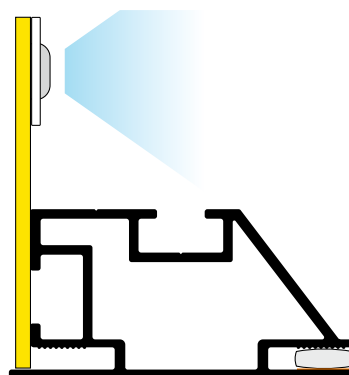
Assembly 1 textile side with backlit LED.
